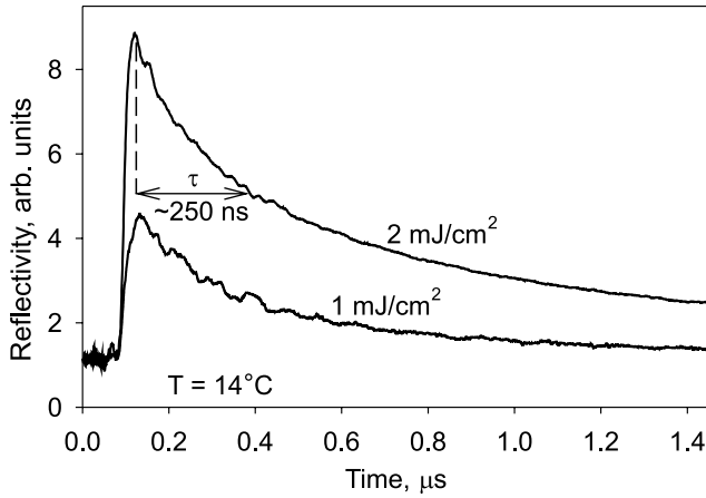
Fig. 2. Dynamics of the change induced in the probe reflectivity of the glass-MgF 2 -composite structure by 6 ns pump pulses ( T = 14^\circ\text{C} , angle of probe incidence \theta = \theta_c ).
