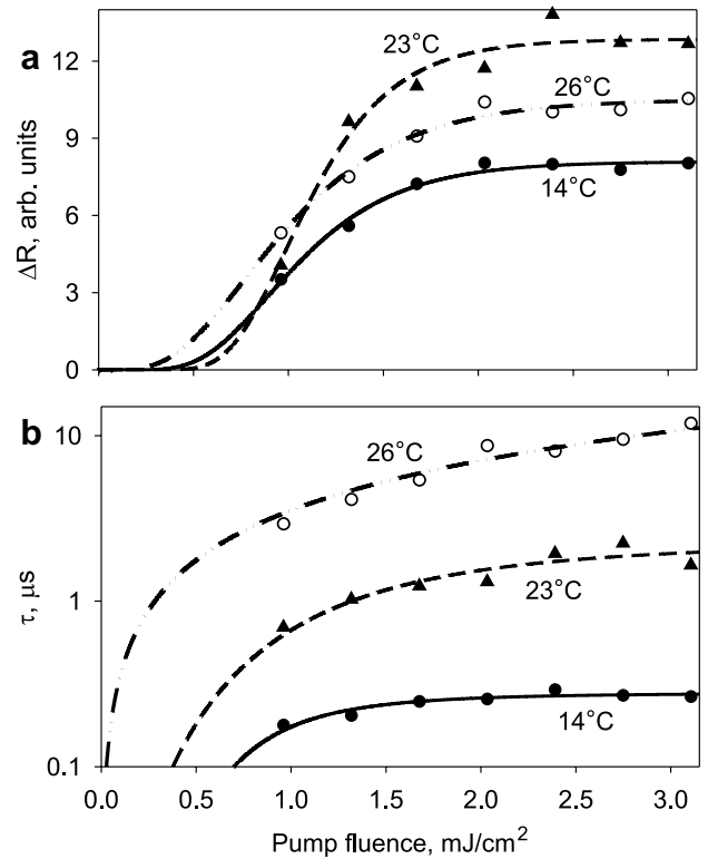
Fig. 4. Dependences on pump fluence of (a) the maximum pump-induced change \Delta R in the reflectivity of the glass-MgF 2 -composite structure, and (b) the corresponding relaxation time \tau , at different sample temperatures.
