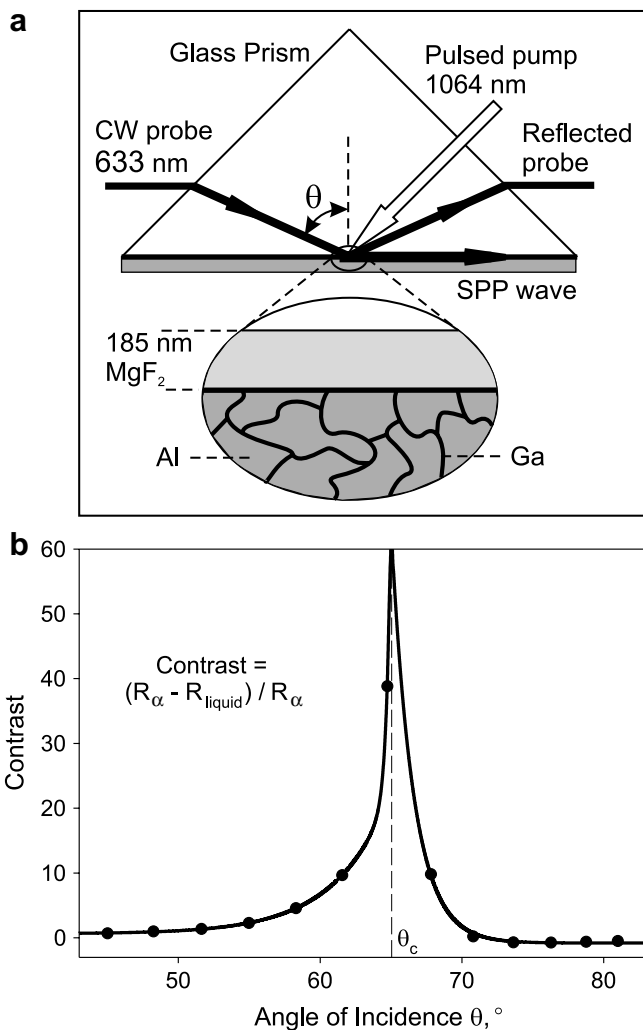
Fig. 1. (a) The arrangement for optical modulation of light-to-SPP wave coupling in the ATR configuration. (b) Angular dependence of reflectivity contrast (defined as [R_\alpha - R_{\text{liquid}}]/R_\alpha where R_\alpha and R_{\text{liquid}} are the \alpha and liquid state reflectivity levels, respectively) for the glass-MgF 2 -Ga/Al composite structure shown in (a). Measurements were made using a p-polarized 633 nm probe beam. The peak position \theta_c \sim 65^\circ is given by that of the minimum in R_\alpha .
