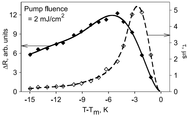
Fig. 3. Temperature dependence of the maximum pump-induced change \Delta R in the glass-MgF 2 -composite structure's reflectivity (closed symbols) and corresponding relaxation time \tau (open symbols) at a pump fluence of 2\text{ mJ/cm}^2 .
